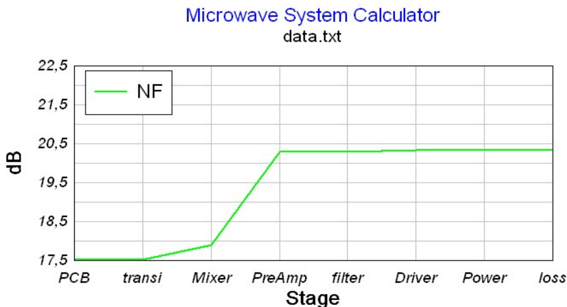
Figure 4: NF resulting from data.txt example PCB stage at 8 dB gain
