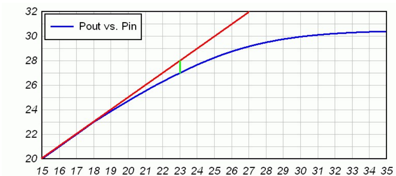
Figure 6: Mystic compression and saturation modeling [dBm both axis]
